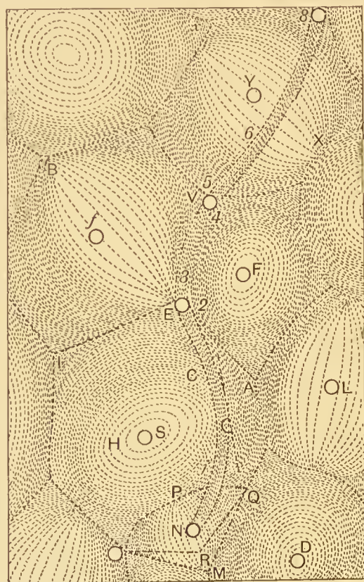
FIG. 55.—Descartes's diagram of vortices, from his Principia .
